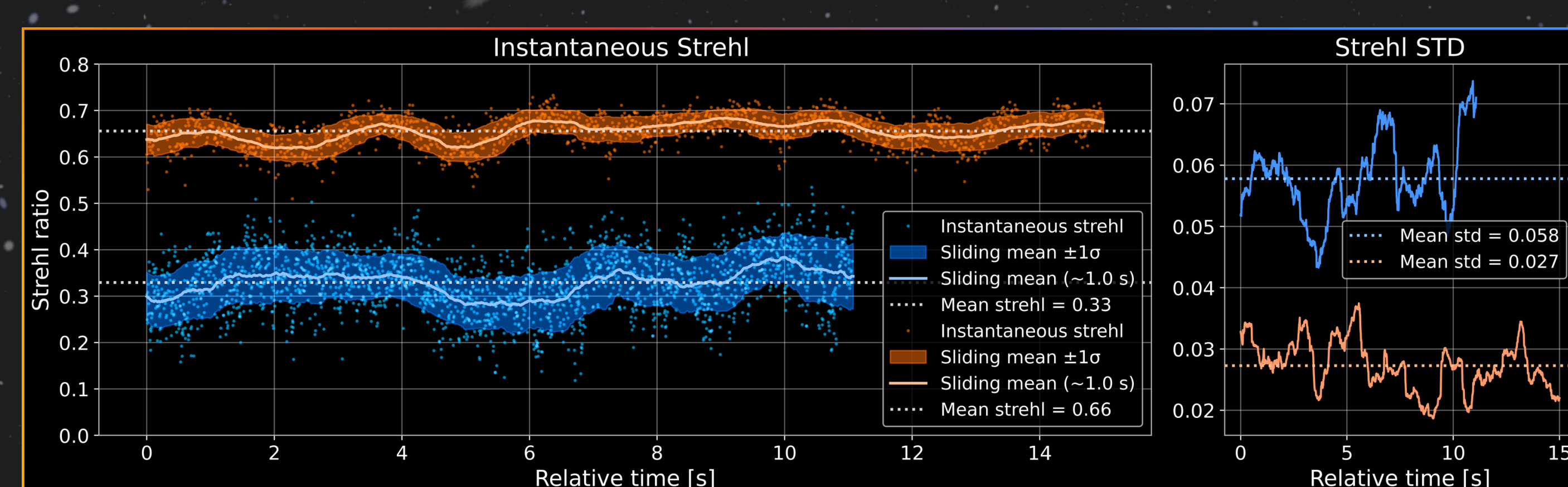
Instantaneous Strehl ratio evolution for March and July 2025 observations.
