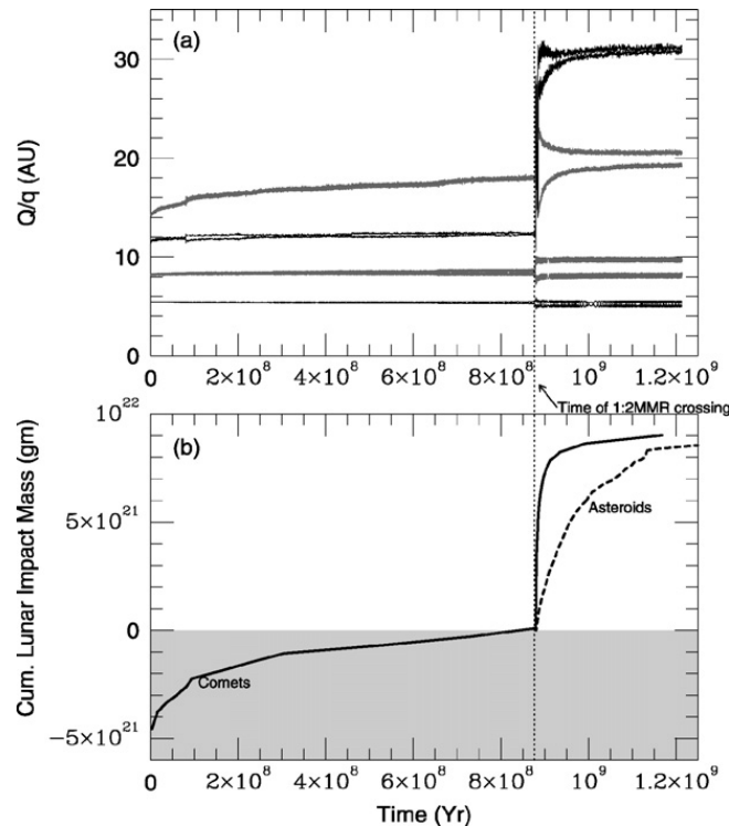
Fig. 2. Planetary migration and the corresponding mass flux towards the inner Solar System, from a representative simulation of [14]. Top: the evolution of the 4 giant planets. Each planet is represented by a pair of curves – the aphelion and perihelion distances. In this simulation Jupiter and Saturn cross their 1/2 mean-motion resonance at 880 My. Bottom: the cumulative mass of comets (solid curve) and asteroids (dashed curve) accreted by the Moon. The comet curve is offset so that the value is zero at the time of 1/2 resonance crossing.
