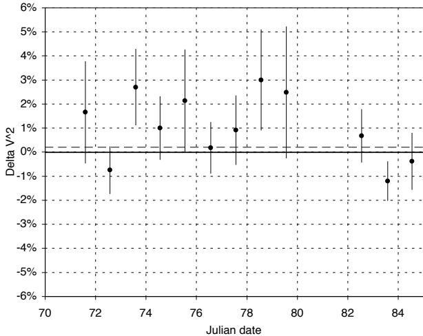
Fig. 4. Observed deviation of the squared visibilities of \delta Eri (B3-D1 baseline only) with respect to the visibility model of a \theta_{UD} = 2.394 mas uniform disk model. The dashed line represents the average deviation over all observations (0.21%).
