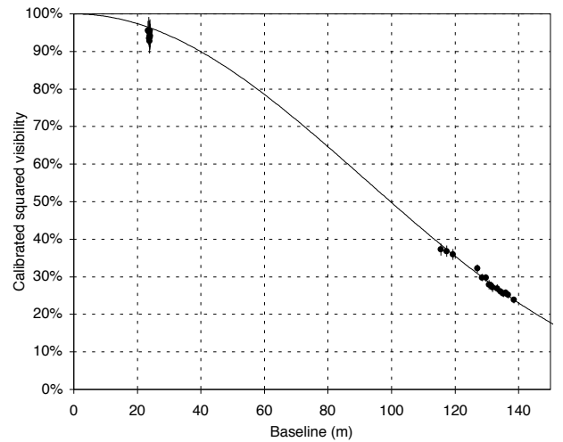
Fig. 2. Squared visibility measurements obtained on \xi Hya. The solid line is a limb darkened disk model with \theta_{LD} = 2.386 \pm 0.009 \pm 0.019 mas (statistical and systematic errors).
