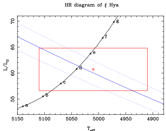
Fig. 8. Zoom of the evolutionary tracks in the H-R diagram for \xi Hya. from label 'a' (509.2 Myr) to 'g' (509.8 Myr), shown by lower case letters and triangles with time steps of 0.1 Myr. Our best model is close to label 'd' at 509.5 Myr (see table 1).
