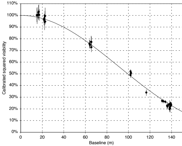
Fig. 1. Squared visibility measurements obtained on \delta Eri. The solid line is a limb darkened disk model with \theta_{LD} = 2.394 \pm 0.014 \pm 0.025 mas (statistical and systematic errors).
